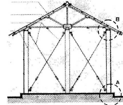
TRANSVERSE SECTION
