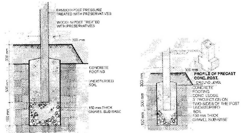
TYPICAL FOOTING FOR TIMBER OR BAMBOO POST
